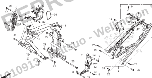
C-39 Chassi
