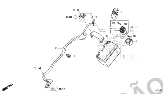
C-39 Chassi
