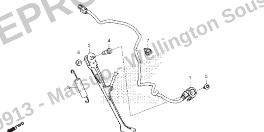
C-31 Cavalete
